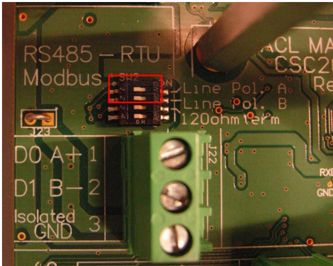
Figure 8 – Line Polarization DIP Switches
