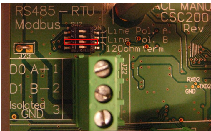
Figure 7 - 120 ohm Termination Resistor DIP Switch
