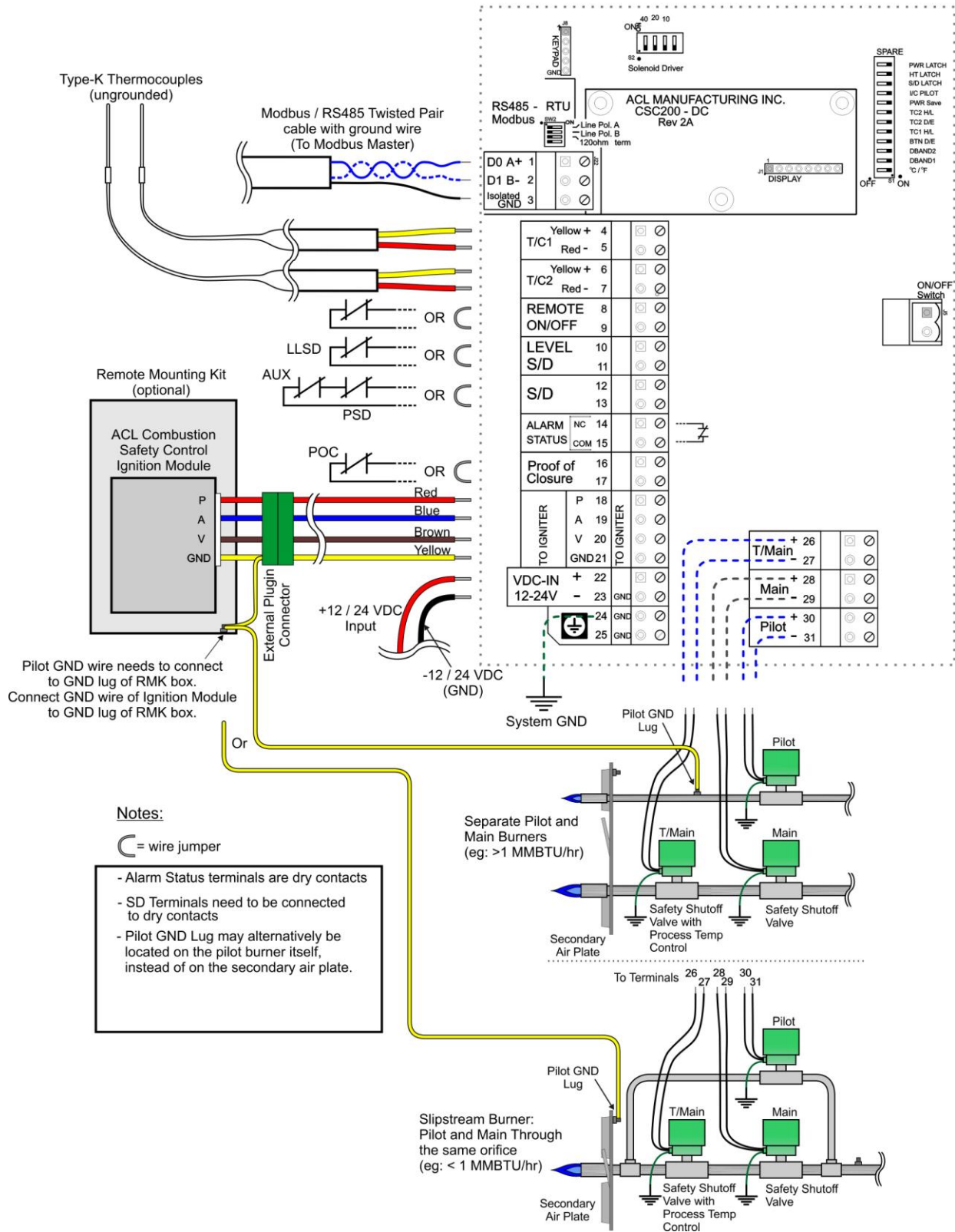
Figure 5 - CSC200 Wiring Diagram
