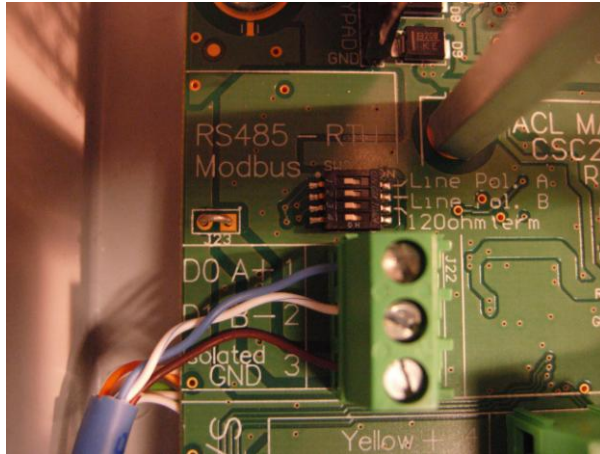
Figure 6 - Example CAT5E Cable Connection
